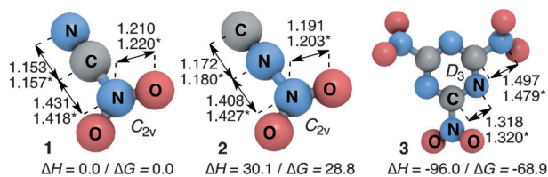
Scheme 1. Nitril cyanide ( 1 ), nitril isocyanide ( 2 ), and 2,4,6-trinitro-1,3,5-triazine ( 3 ). Relative enthalpies and Gibbs free energies were calculated at the M06-2X/cc-pVTZ level of theory (kcal mol -1 , 1 atm, 298 K). Geometries [Å] were determined by M06-2X/cc-pVTZ and RI-B2PLYP/def2-TZVPP (*) optimizations.
